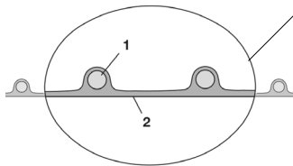
Profile 1. Semi-rigid, crush resistant PVC spiral 2. Layer of polyurethane
